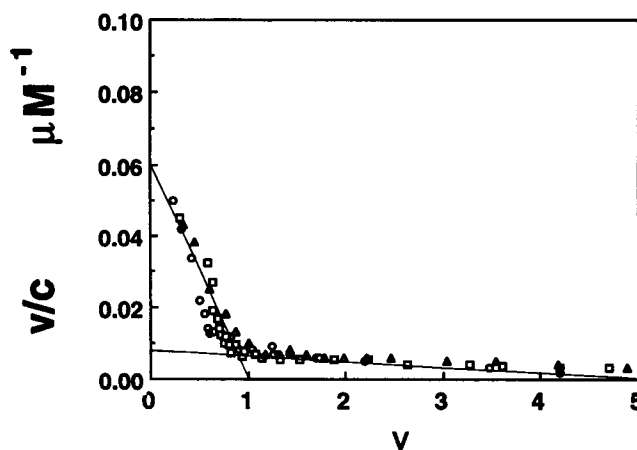
FIGURE 2 Scatchard plot for \text{Ca}^{2+} titration of deionized bO sample. The slope of each straight line gives the binding affinity of \text{Ca}^{2+} , and the x-intercept shows the number of \text{Ca}^{2+} in each category. C is the concentration of free calcium ions in equilibrium with the bO solution; V = [\text{bound } \text{Ca}^{2+}]/[\text{bO}] , where [\text{bound } \text{Ca}^{2+}] is the concentration of bound \text{Ca}^{2+} and [\text{bO}] is the concentration of deionized bO. The data of three experiments ( \square , \Delta , \circ ) are plotted to show the reproducibility. The fact that the plot is different from that in bR and monomer bR (Fig. 1) suggests that the high affinity sites are not far from retinal.
