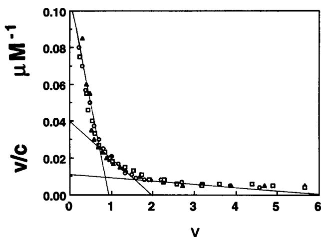
FIGURE 1 Scatchard plot for \text{Ca}^{2+} titration of deionized monomer bR. The slope of each straight line gives the binding affinity constant of \text{Ca}^{2+} , and the x-intercept shows the number of \text{Ca}^{2+} in each class. C is the concentration of free calcium ions in the monomer bR solution; V = [\text{bound } \text{Ca}^{2+}]/[\text{bR}] , where [\text{bound } \text{Ca}^{2+}] is the concentration of bound \text{Ca}^{2+} and [\text{bR}] is the concentration of deionized monomer bR. The data of three experiments ( \square , \Delta , \circ ) are plotted to show the reproducibility. The similarity of the plot to that for deionized bR suggests that 1) the curvature in the Scatchard plot is not due to cooperativity between sites on different monomers, and 2) the metal cation binding sites reside within the monomer bR and not between bR monomers.
